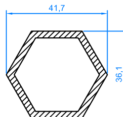
Hexagonal tubes in C35E Tubes 6 pans en C35E
