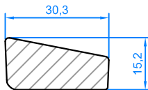
Key section for storage equipment Profil clavette
