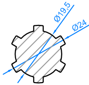
Splined shaft for power transmission Arbre cannelé Transmission
