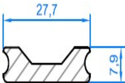
Profil chariot Linear bearing carrier Profilschiene
