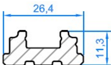
Profil chariot Carriage section Profilschiene
