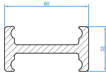
Linear ball rail Rail de guidage
