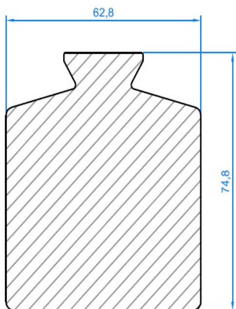
Barreau clavette Keybars Keilstab
