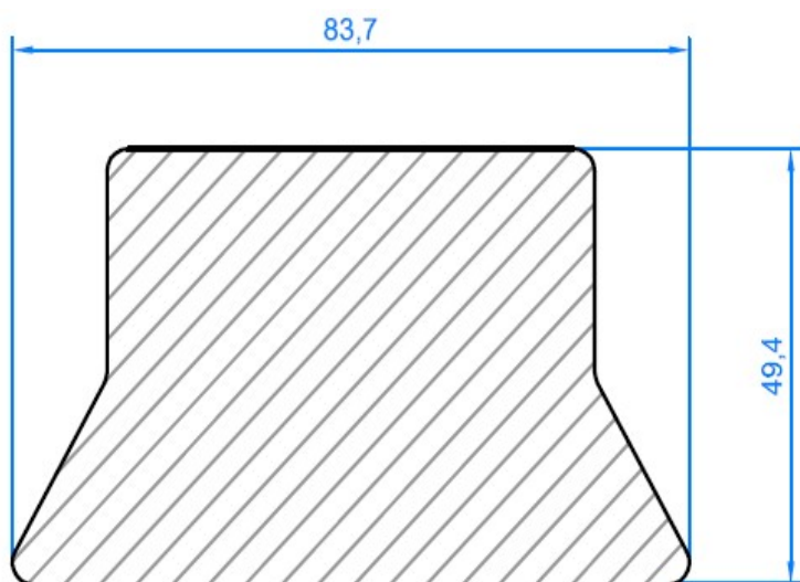
Barreau clavette Connecting keybars Keilstab
