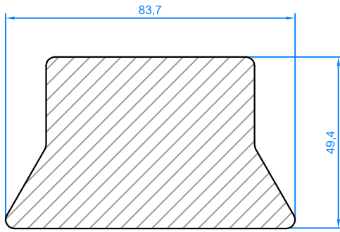
Connecting keybars Barreau clavette
