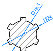
Splined shaft Arbre cannelé
