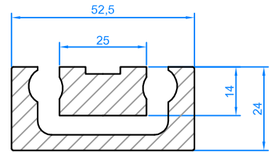
Train door track Guidage porte de train
