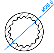
Steering column splined tube Tube cannelé colonne de direction
